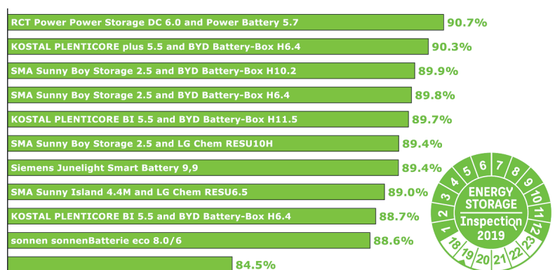
Figure 2: The results of the ENERGY STORAGE Inspection 2019. The majority of systems achieved a very good SPI above 88%.
